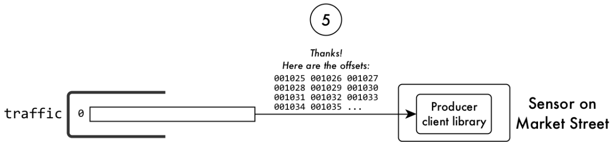
Figure 8: The server acknowledges receiving the messages
