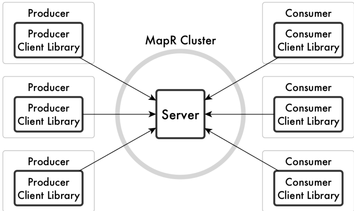
Figure 5: The relationship of the HPE Data Fabric Streams server to producers, consumers, and client libraries
