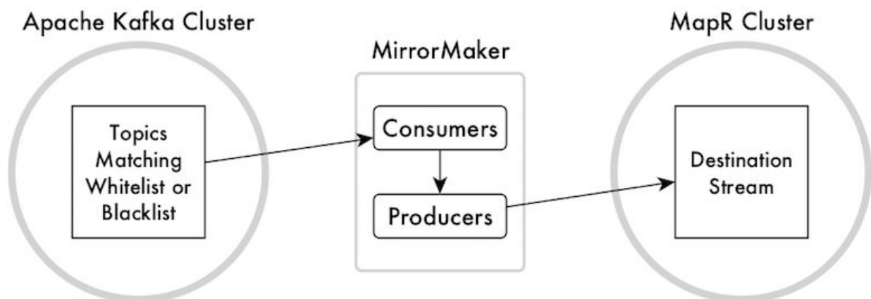
Figure 22: Mirroring from Apache Kafka to HPE Data Fabric Streams
