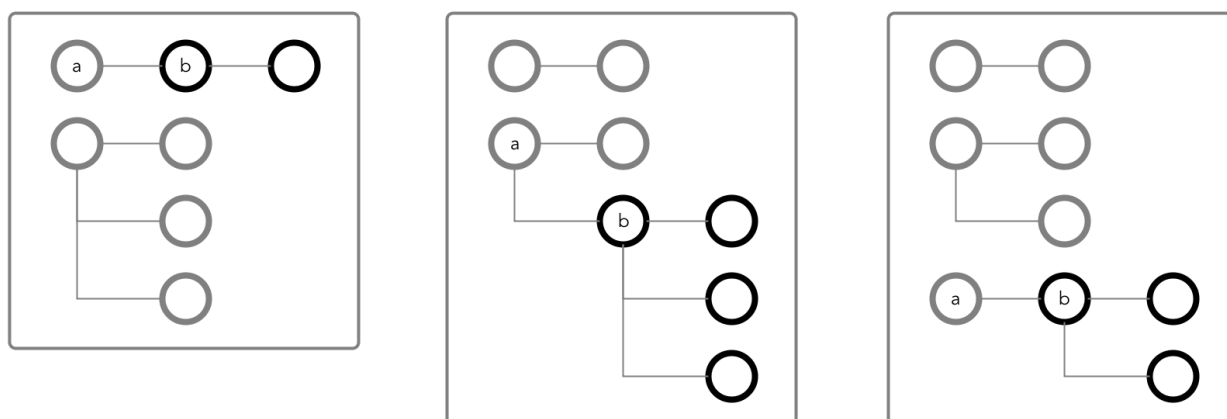
Figure 3: The three JSON documents with column family CF1 in black
