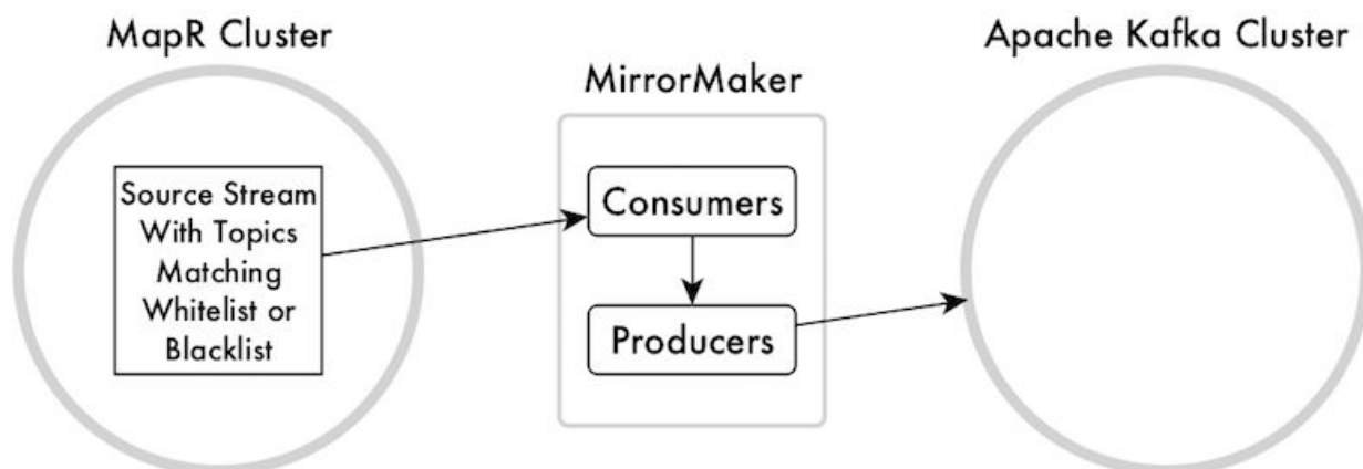
Figure 23: Mirroring from HPE Data Fabric Streams to Apache Kafka
